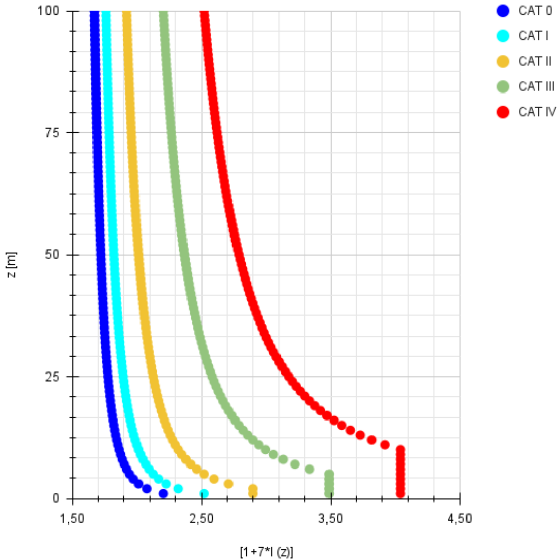
Figure 2: turbulent factor [1 + 7 I_v(z)]
